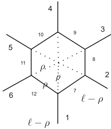
Figure 5: Graph with 'critical' edge degree 6
