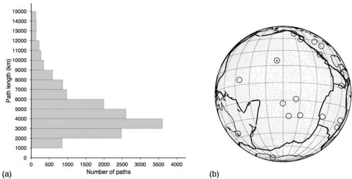
Figure 5. (a) Histogram of path lengths within the clustered data set. (b) Voronoi diagram in the style of Debayle & Sambridge (2004) for our clustered data set.
