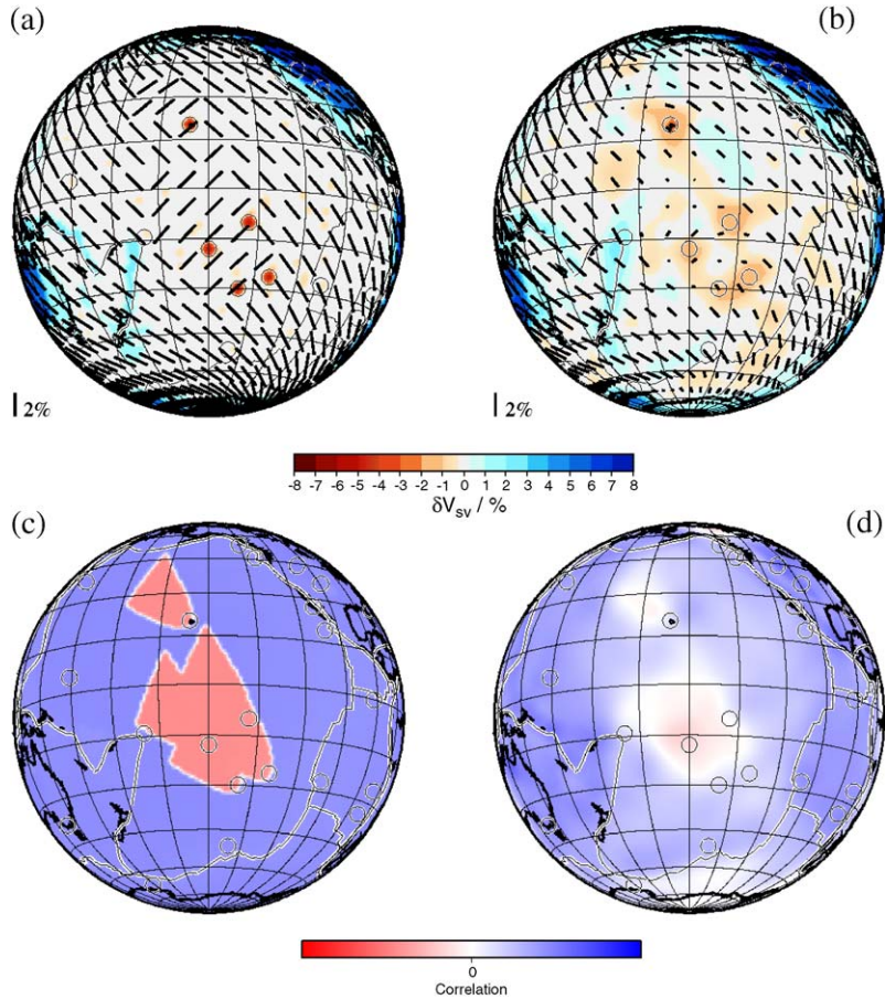
Fig. 10. Synthetic tests for the recovery of plume-related disturbances in azimuthal anisotropy: (a) synthetic input model with uniform 2% NW-trending anisotropy, 5 plumes of radius 200 km and 5% shear wave anomaly, and parabolic regions of rotated anisotropy; (b) output of the synthetic test; (c) input model plotted as correlation with respect to a ‘plate motion’ (velocity 100 mm/yr) parallel to the background anisotropy; (d) correlation of the output model with the same ‘plate motion’.
