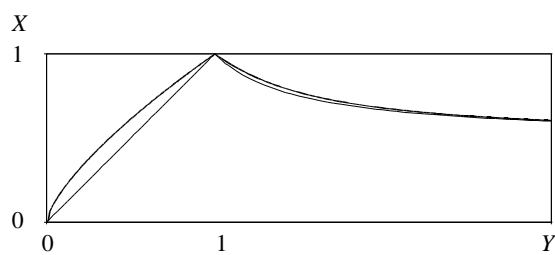
Figure 3: Graph of the optimal solution h(Y) (thick) and graph of the proposed solution (thin) in the case \beta' > 0 .
