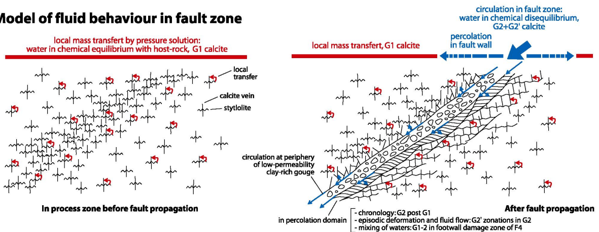
Fig. 3. Models of structural development and fluid behaviour in normal fault zones affecting carbonates in the Aigion area. See comments in the text.
