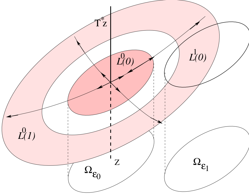
FIGURE 4.1. Sketch of the Lagrangian manifolds \mathcal{L}_{\eta_1}^0(0) situated above \Omega_{\epsilon_0} and centered at z (center ellipse, dark pink), its image \mathcal{L}_{\eta_1}^0(1) through the flow (external annulus, pale pink) and the intersection \mathcal{L}_{\eta_1}^1(0) of the latter with T^*\Omega_{\epsilon_1} . The thick arrows show the possible momenta at points x \in M .
