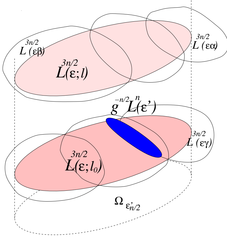
FIGURE 4.2. Decomposition of (g^{n/2}\mathcal{L}^n(\epsilon)) \cap T^*\Omega_{\epsilon'_{n/2}} into connected leaves (here we show two of them, in pink). The leaf \ell contains the components \mathcal{L}^{\frac{3}{2}n}(\epsilon\alpha) , \mathcal{L}^{\frac{3}{2}n}(\epsilon\beta) while the leaf \ell_0 contains \mathcal{L}^{\frac{3}{2}n}(\epsilon\gamma) . We also show the elongated leaf g^{-n/2}\mathcal{L}^n(\epsilon') supporting the state w^{n/2}(\epsilon') (in blue). This state might interfere with v^{\frac{3}{2}n}(\epsilon, \ell_0) , but not with v^{\frac{3}{2}n}(\epsilon, \ell) or any other leaf above \Omega_{\epsilon'_{n/2}} .
