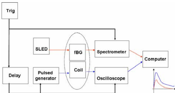
Figure 7 - Schematics data acquisition chain
