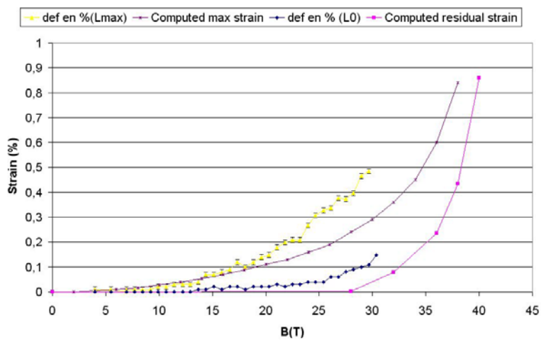
Figure 9 - Fem vs Measurement
