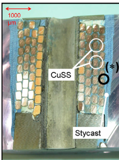
Figure 4 - Test coil section
