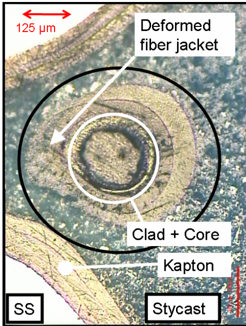
Figure 5 - Implemented fiber behaviour
