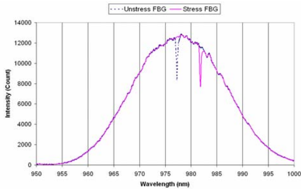
Figure 2 - Typical transmission spectrum through our FBG in the unstrained and an axially strained state
