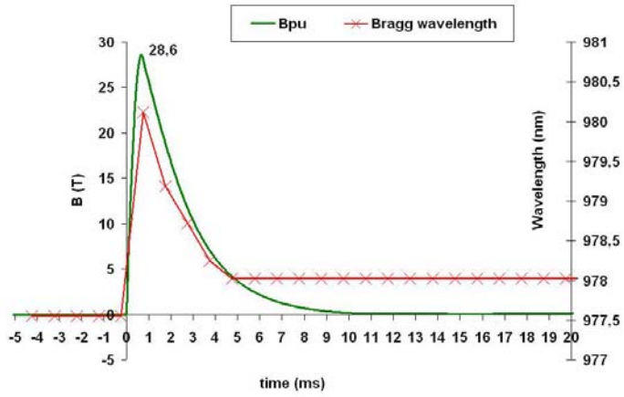
Figure 8 - Field and Bragg wavelength shift
