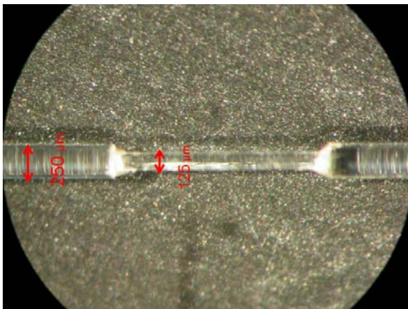
Figure 6 - Stripped fiber
