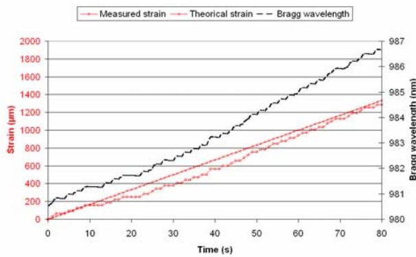
Figure 3 - Bragg resonance shift
