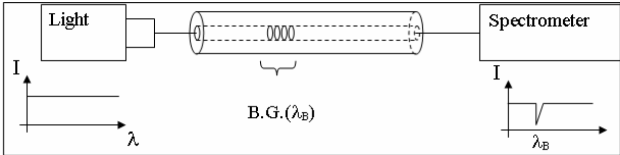
Figure 1 - Fiber Bragg grating effect
