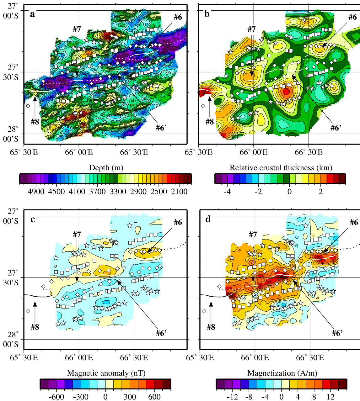
Figure 4. (a) Bathymetric map, (b) crustal thickness variation map, (c) magnetic anomaly map, and (d) magnetization distribution of survey box C along the SWIR between 65°30'E and 67°E. Same caption as in Figure 2 except that magnetic anomaly picks are from Cannat et al. [2003].
