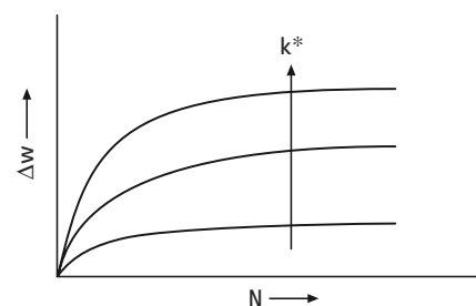
Figure 5. Theoretical evolution of the mesoscopic dissipated energy per cycle versus the number of test cycles (in the case of uniaxial loading)
