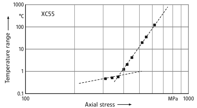
Figure 7. Evolution of the stabilized temperature versus the macroscopic load for a rotating bending test on an XC55 steel after Luong's results [27]
