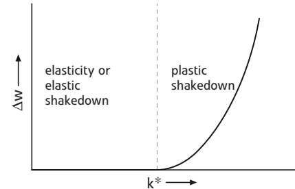
Figure 4. Theoretical evolution of the mesoscopic dissipated energy per cycle versus the macroscopic load (in the case of uniaxial loading)
