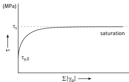
Figure 1. Schematic hardening curve of a mono crystal under cyclic loading. \tau is the resolved shear stress acting on the gliding plane and \tau_{y,0} , the initial yield limit value. \tau_s is the saturation stress and \Sigma|\gamma_p| the cumulated plastic shear.
