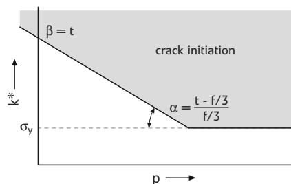
Figure 2. Graphical representation of the Papadopoulos HCF criterion. t and f are, respectively, the fatigue limit in torsion and in bending. \sigma_y is the initial yield limit in tension of the crystal.
