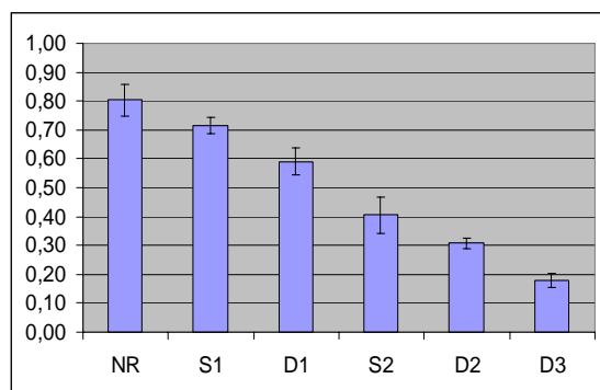
Figure 1: Global preference rates for each system. (Error marks are confidence intervals)
