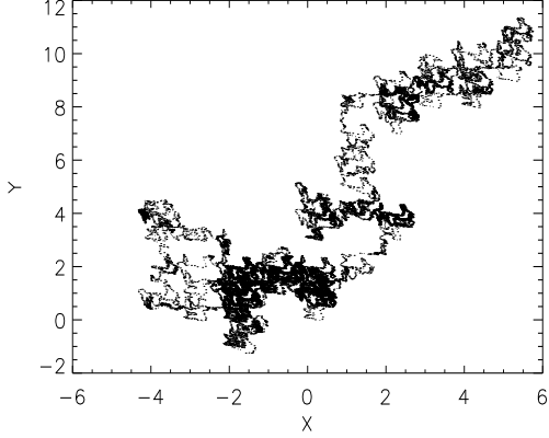
Figure 1: Poincaré surface of section of a trajectory obtained from the starting Hamiltonian (4) assuming a = 0.8 (weakly chaotic region).
