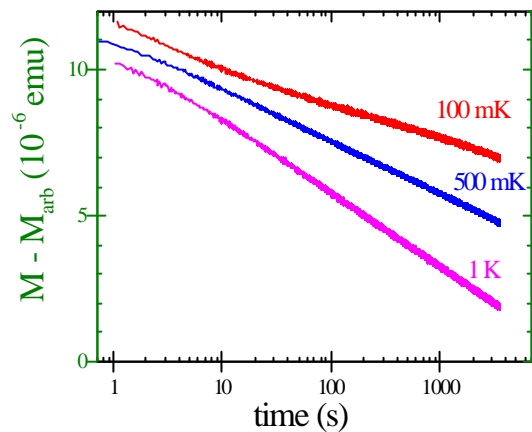
Fig. 1. Example of relaxation curves as measured on one of our samples ( \alpha\text{-Fe}_2\text{O}_3 nanoparticles) after switching off a 60 Oe magnetic field.
