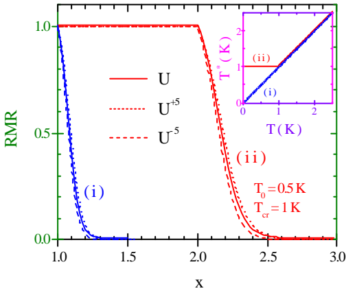
Fig. 4. Calculated RMR( x ) for (i) thermally activated dynamics and (ii) quantum dynamics (in the plateau hypothesis with an arbitrary choice of T_{cr}=1K and T_0=0.5K ). The corresponding effective temperatures are plotted in the insert. Three choices of P(U)\Delta m(U) are represented.
