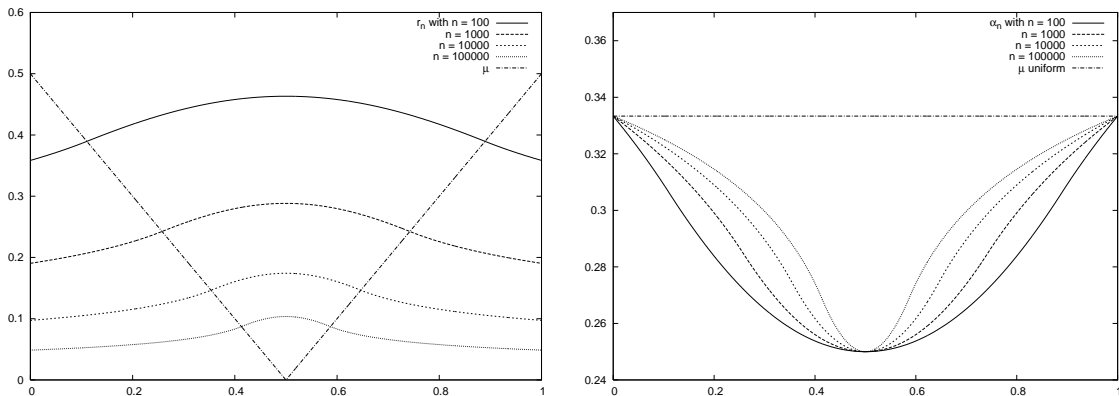
FIGURE 1. r_n(\cdot) and \alpha_n(\cdot) for several sample sizes
