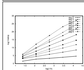
Figure 8: Exponential model: Convergence of the k_{min} estimate wrt h , approximation fitting
