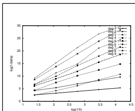
Figure 5: Exponential model: Convergence of the normal estimate wrt h , interpolation fitting
