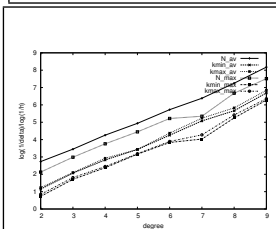
Figure 12: Exponential model: Convergence of normal and curvature estimates wrt the degree of the approximation fitting
