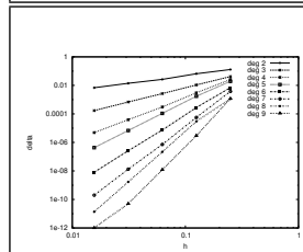
Figure 10: Exponential model: Convergence of the k_{max} estimate wrt h , approximation fitting
