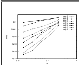
Figure 9: Exponential model: Convergence of the k_{max} estimate wrt h , interpolation fitting
