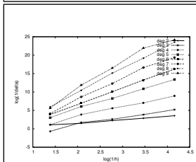
Figure 7: Exponential model: Convergence of the k_{min} estimate wrt h , interpolation fitting
