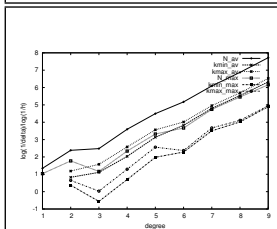
Figure 11: Exponential model: Convergence of normal and curvature estimates wrt the degree of the interpolation fitting
