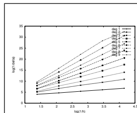
Figure 6: Exponential model: Convergence of the normal estimate wrt h , approximation fitting
