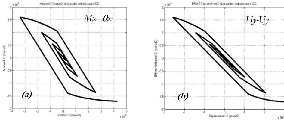
Figure 5.11. Cyclic behaviour considering rocking of the foundation.
