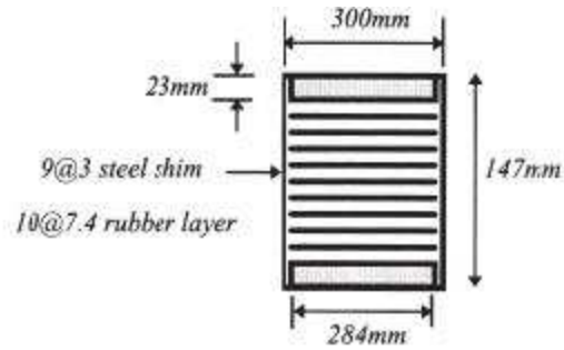
Figure 6.2. Details of the base isolator [Chung et al., 1999]
