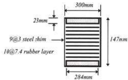
Figure 6.2. Details of the base isolator [Chung et al., 1999]
