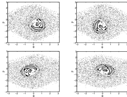
Figure 2. Phase space of the N particles at t = 400, 401.25, 402.5 and 403.75 .
