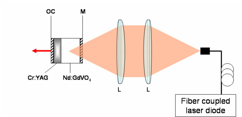
Fig.1 : experimental setup.
