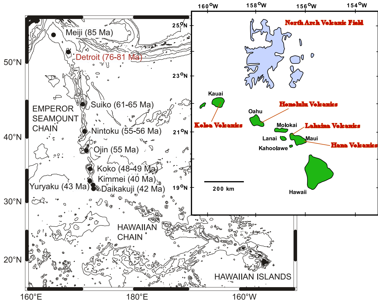
Figure 1. Map showing volcanoes along the Emperor Seamount Chain (eruption ages within parentheses). Inset shows the Hawaiian Islands and locations of rejuvenated-stage and North Arch lavas that have been analyzed for Hf isotopic ratios. Figure is modified from Dixon and Clague [2001] and Regelous et al. [2003] by adding Ar-Ar ages for Emperor Seamounts from Sharp and Clague [2002] and Duncan and Keller [2004].
