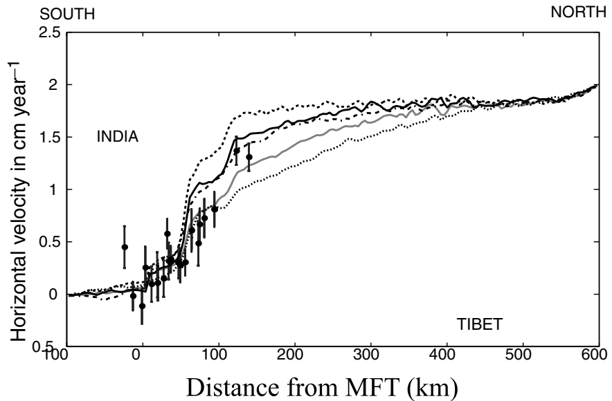
Figure 9. (a) Influence of ramp slope on horizontal velocities for centre Nepal. (b) Influence of northern flat slope on horizontal velocities for centre Nepal. Measured horizontal velocities come from GPS measurements of Jouanne et al. (2003) expressed in the India fixed reference frame with 95 per cent confidence error bars.
