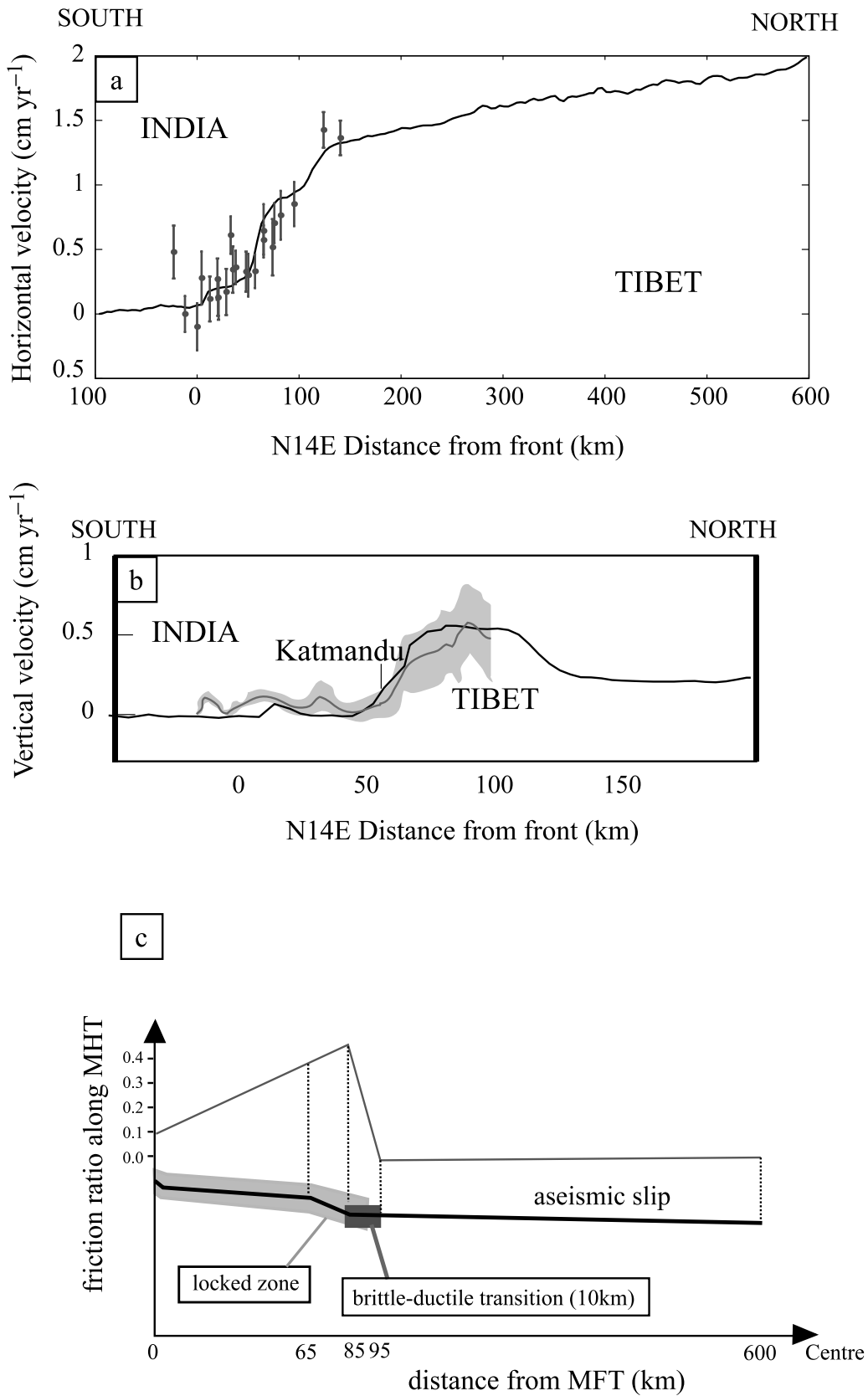
Figure 11. (a) Calculated (lines) and measured (full circle) horizontal interseismic velocities for final centre Nepal model. Measured velocities come from GPS measurements of Jouanne et al. (2003) expressed in the India fixed reference frame with 95 per cent confidence error bars; (b) Calculated (black lines) and measured (grey area) vertical interseismic velocities for final centre Nepal model. Measured velocities come from levelling measurements of Jackson & Bilham (1994); (c) MHT friction ratios for final central model accordingly with the distance from the MFT.
