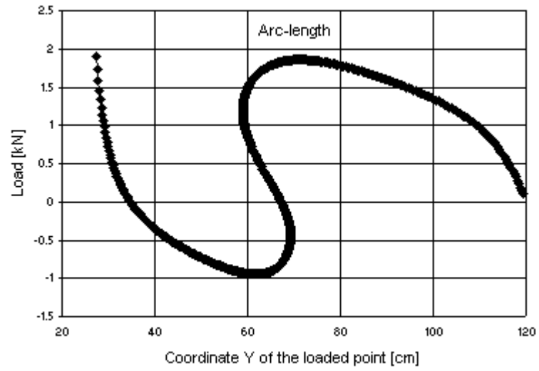
FIGURE 22. The Lee frame: Load-coordinate curve of the loaded point (Arc-length method).
