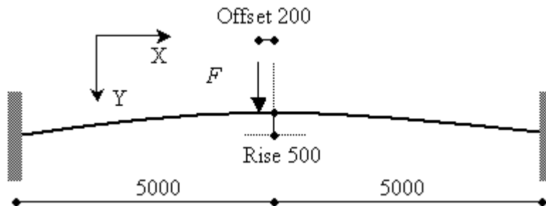
FIGURE 23. Swallow circular arch subject to near central point load.
