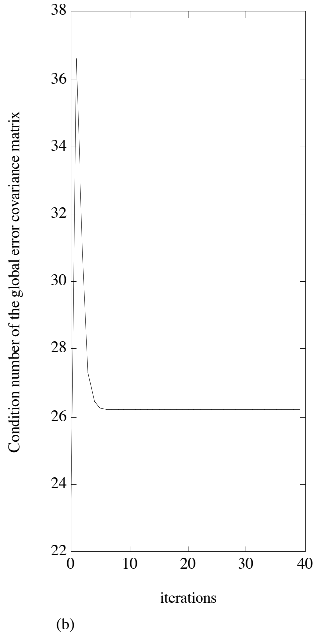
Fig. 8: Effect of round-off errors on Algorithm 4.2 when the local measurements are not scalar.
