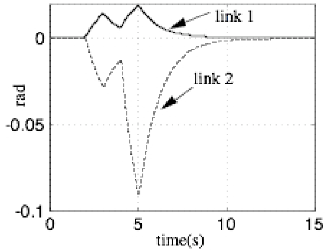
Figure 5: Position errors, links 1 and 2.
