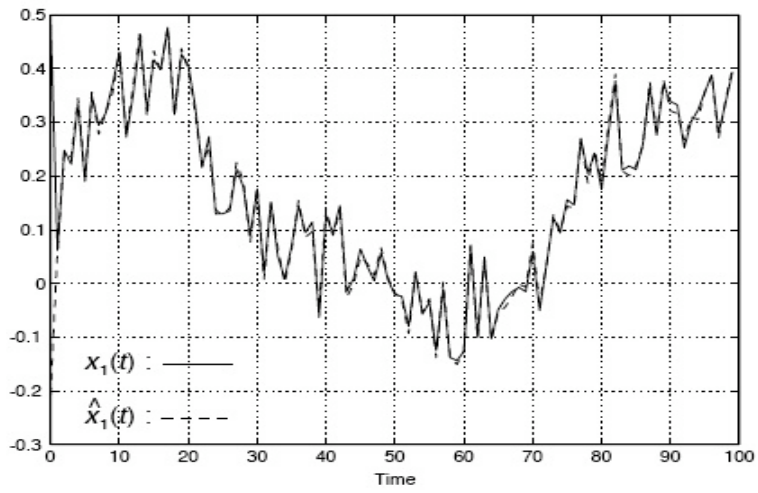
Figure 2: Actual state x_1(t) and estimated state \hat{x}_1(t) .
