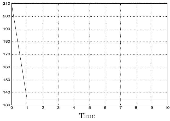
Figure 4: Trace of the estimation covariance P(t) .
