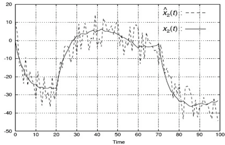
Figure 3: Actual state x_2(t) and estimated state \hat{x}_2(t) .
