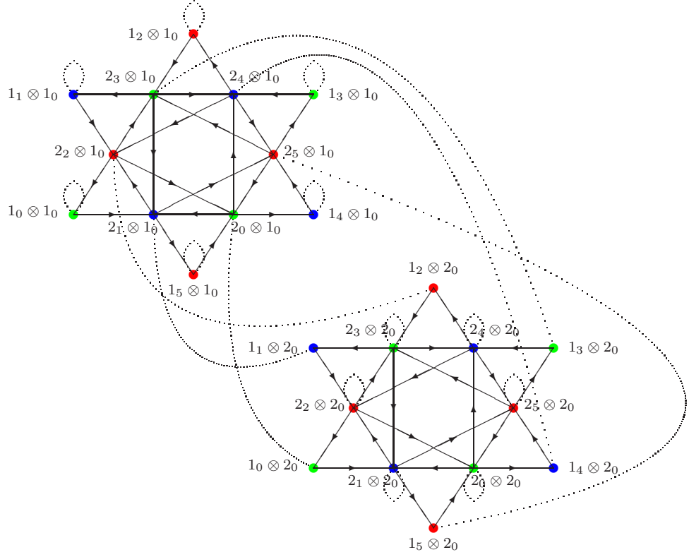
Figure 3: Occeanu graph Oc(\mathcal{E}_5^*) . The two left chiral generators are 2_1 \otimes 1_0 and 2_2 \otimes 1_0 , the two right chiral generators are 1_1 \otimes 2_0 and 1_2 \otimes 2_0 .
