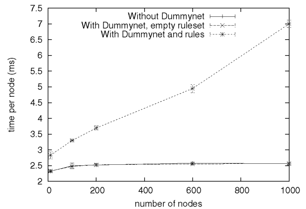
Figure 7. Overhead caused by Dummynet in a token ring
