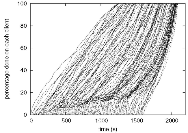
Figure 8. Evolution of the download of the 160 clients.
