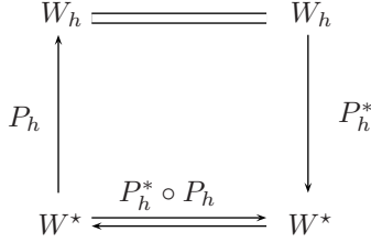
Figure 1: Commutative diagram
