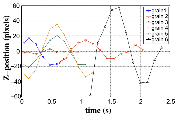
FIG. 6: (Color online) Oscillation of 6 dust grains 10 seconds after plasma extinction. Non oscillating dust grain and opposite phase oscillations are observed.
