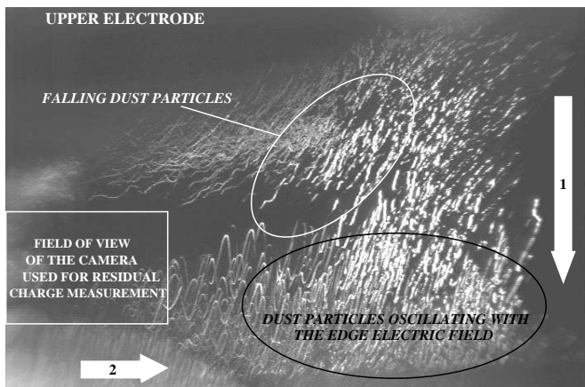
FIG. 4: Superimposition of video frames taken with a large field of view CCD camera. Arrows 1 and 2 represent respectively the vertical and the horizontal components of the temperature gradient. Edge effects as well as falling dust particles can be seen.
