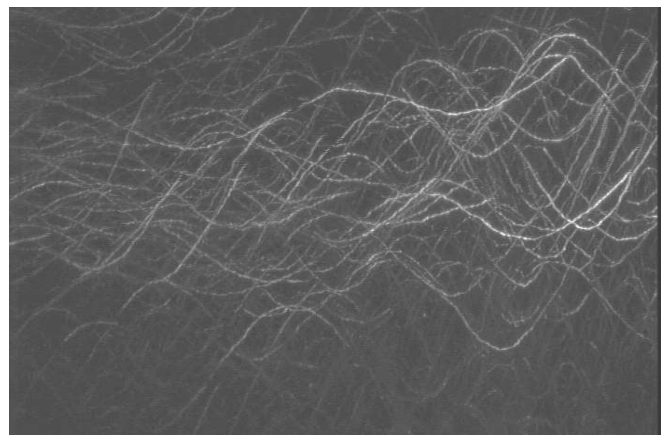
FIG. 5: Superimposition of video frames 10 seconds after plasma extinction. Dust particle oscillations can clearly be seen. The temperature gradient has a slight horizontal component. Therefore, oscillations are in the 2D laser plane.
