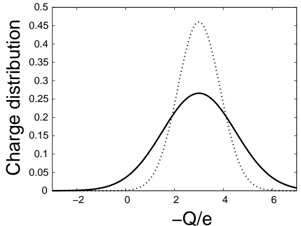
FIG. 9: Charge distribution with and without image force correction. Dotted line represents distribution with \Delta Q = 0.5\sqrt{Q} . Solid line represents distribution with \Delta Q = 0.87\sqrt{Q} [37].
