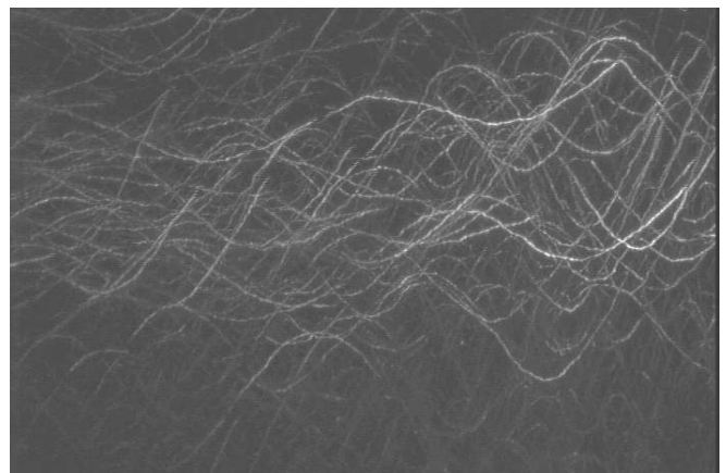
FIG. 5: Superimposition of video frames 10 seconds after plasma extinction. Dust particle oscillations can clearly be seen. The temperature gradient has a slight horizontal component. Therefore, oscillations are in the 2D laser plane.
