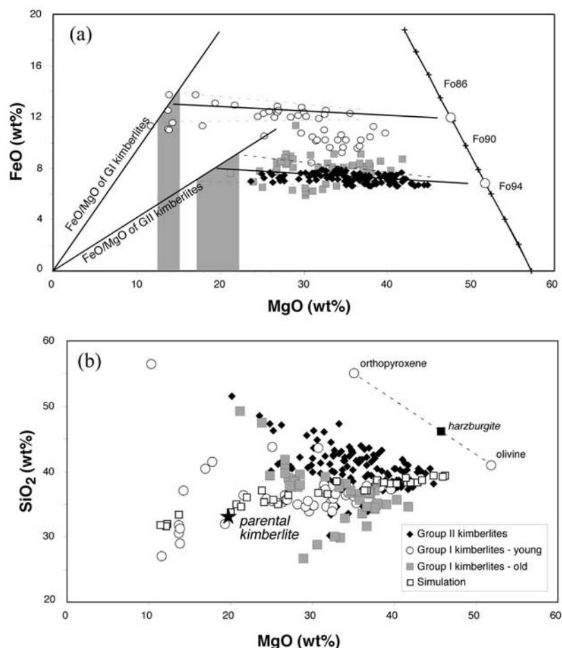
Figure 4. (a) MgO versus FeO in kimberlites and in olivine. For the whole rock compositions 0.85 \cdot \text{FeO}(\text{tot}) is plotted on the assumption that 15% of the iron is \text{Fe}^{3+} . Kimberlites from the Kaapvaal craton plot on an olivine control line that projects to \text{Fo}_{93} , a composition like that recorded in peridotite xenoliths from the Kaapvaal lithospheric mantle; kimberlites from younger cratons project to less magnesian olivine compositions. The sloping lines represent the FeO/MgO ratios of liquid in equilibrium with \text{Fo}_{93} for the Kaapvaal kimberlites and with \text{Fo}_{86.5} for the younger kimberlites. The intersections of these lines with the kimberlite data give the MgO contents of the parental kimberlitic liquids, as shown with the grey fields. Data are from the compilation of published and unpublished sources of C. B. Smith. (b) MgO versus \text{SiO}_2 . The data project to the compositions of olivine and not to a mixture of olivine and orthopyroxene, as exists in lithospheric mantle. The trend labeled “Simulation” was calculated in the following way. First, a mixture of 2/3 olivine and 1/3 orthopyroxene was added to a hypothetical parental kimberlite liquid containing 33% \text{SiO}_2 and 20% MgO to simulate the assimilation of lithospheric harzburgite. Both olivine and orthopyroxene had \text{Mg}/(\text{Mg} + \text{Fe}) = 0.93 ; the amount added varied randomly between 5 and 35%. Then 5 to 85% of olivine with the composition \text{Fo}_{93} was added or subtracted to simulate the accumulation or fractionation of olivine into or from the hybrid liquid. The simulated trend corresponds to that of the Kaapvaal (Group II) kimberlites.
