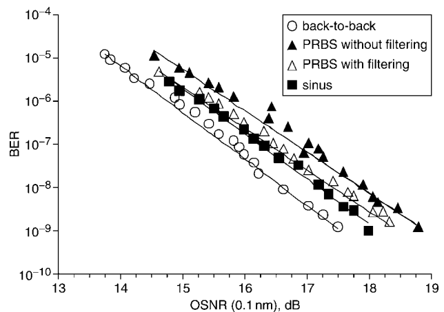
Fig. 2 OSNR penalty induced by three different modulation formats of pump phase
