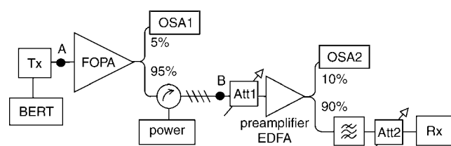
Fig. 1 Experimental setup for BER measurements
