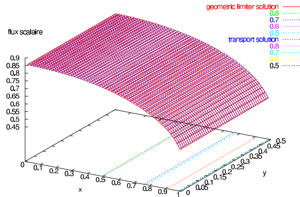
Figure 13: transport versus geometric limiter
