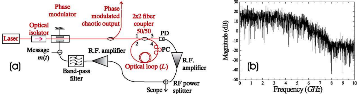
Fig. 12. High dimensional, high speed, phase chaos: (a) experimental setup; (b) RF spectrum of the electronic feedback signal.
