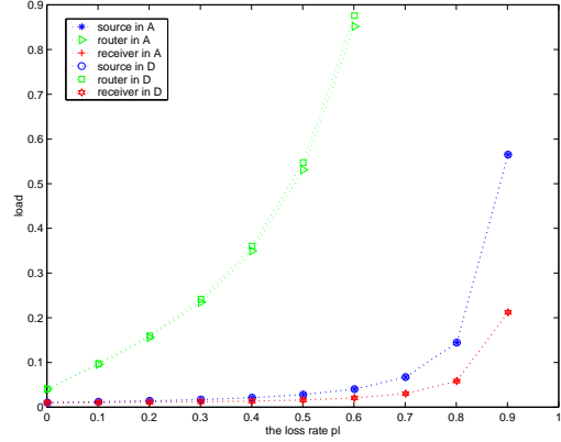
Figure 9: Load at the different nodes with 5 receivers (a) \lambda = 0.001 (b) \lambda = 0.01 .
