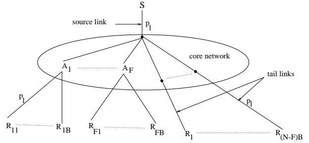
Figure 1. Network Model.
