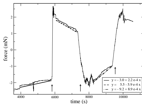
Figure 4. Force evolution for an old foam. The bead is at rest, excepted for the three modifications of the foam loading, indicated by arrows. Between these small bead translations the foam creeping motion is observed.
