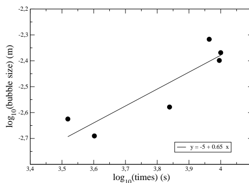
Figure 5. Evolution of the bubble diameter with time. Despite the small parameter range, a logarithmic plot is displayed with a slope compatible with the power law prediction d \sim t^{0.5} in scale invariant coarsening regime.
