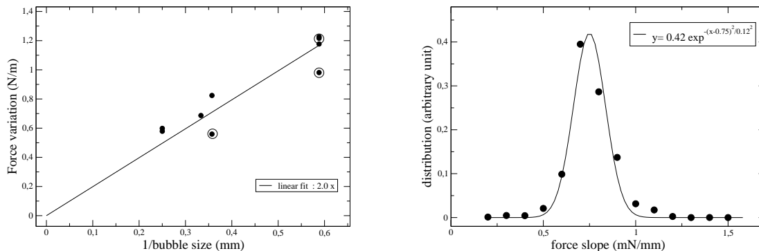
Figure 2. (a) Force derivative during elastic loading with respect to the cell displacement, for various bubble sizes. The open circles indicate a box moving downwards. (b) Force slope distribution in a 3mm bubbles foam. This distribution, fitted by a Gaussian curve, is due to the experimental noise but also to the intrinsic local fluctuations of the foam properties.
