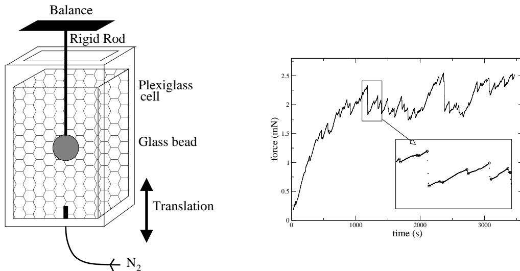
Figure 1. (a) Experimental set-up. (b) Typical force graph obtained with the foam moving at 5 \mu\text{m/s} downwards (positive forces are oriented downwards). The circle on the enlarged graph indicate the force extrema and the small dots the discrete measure points.
