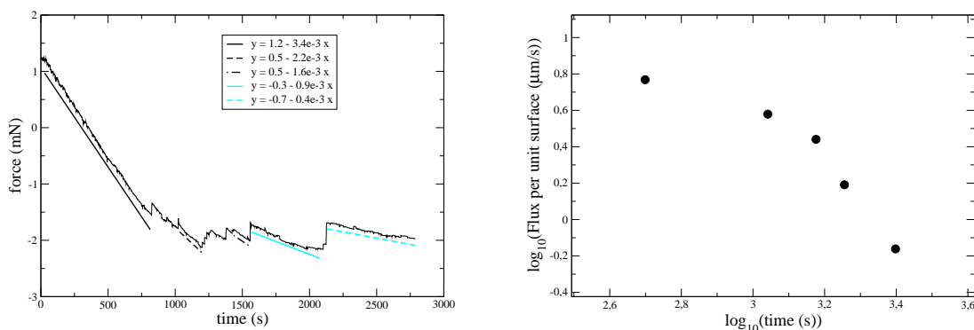
Figure 3. (a) Force signal obtained for a young foam with bubble diameter 3 mm, when the bead is at rest. The slow force decreases are fitted by linear laws. (b) Evolution of the solution flux induced by gravity drainage, deduced using eq. 1 from the slopes of the linear fit given on graph (a).
