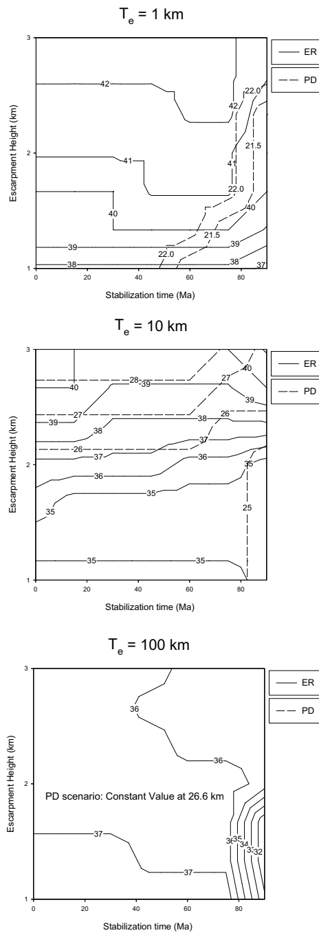
Figure 6: Distance from the coast to x_a , the location where the minimum age is predicted, as a function of escarpment height, h_0 , and stabilization time, t_s , for three values of the assumed elastic plate thickness, T_e .
