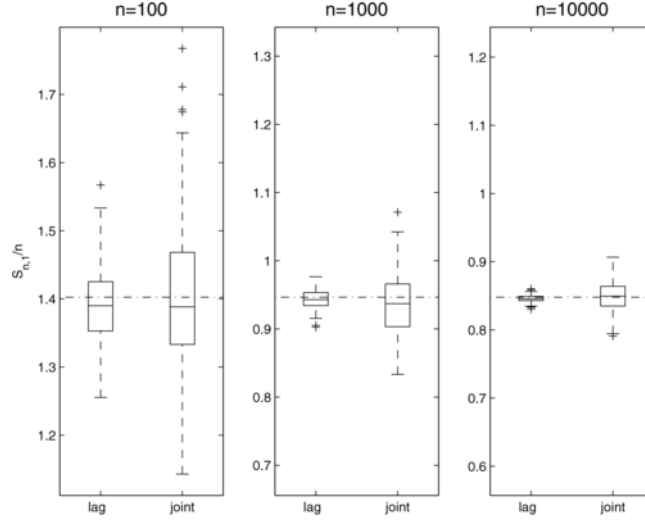
Figure 3. Boxplots of estimates of \phi_{\nu,0:n|n}S_{n,1}/n , produced by means of both the fixed-lag technique and standard trajectory-based smoothing, for the noisily observed AR(1) model in Example 4.1. Each box is based on 200 estimates, and the size of the particle population was N = 1000 for all cases.
