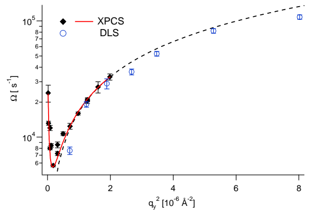
FIG. 4: (Color online) Comparison between the XPCS and DLS results. Diamonds and solid line: XPCS data and fit (as in Fig. 3). Dotted line: high- q_{\perp} extrapolation of the fit. Open dots: DLS results.
