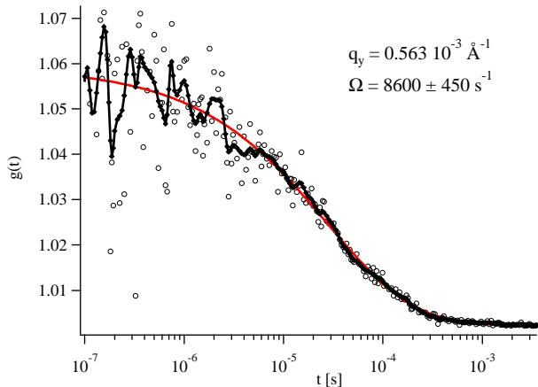
FIG. 2: (Color online) Correlation function g(t) measured for ( q_{\perp} = 0.563 \cdot 10^{-3} \text{ \AA}^{-1} ). Open symbols: raw signal; dots and solid line: smoothed signal; solid line: fit with the model described in the text (equation 3).
