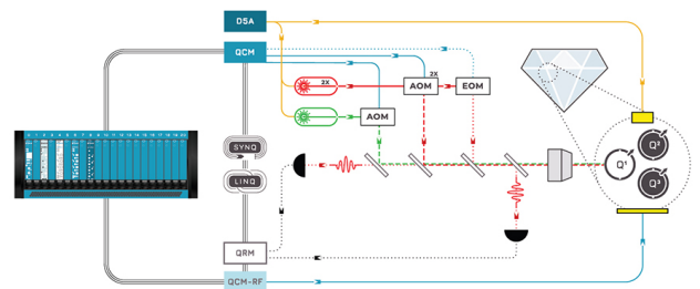
NV-Centers Setup
