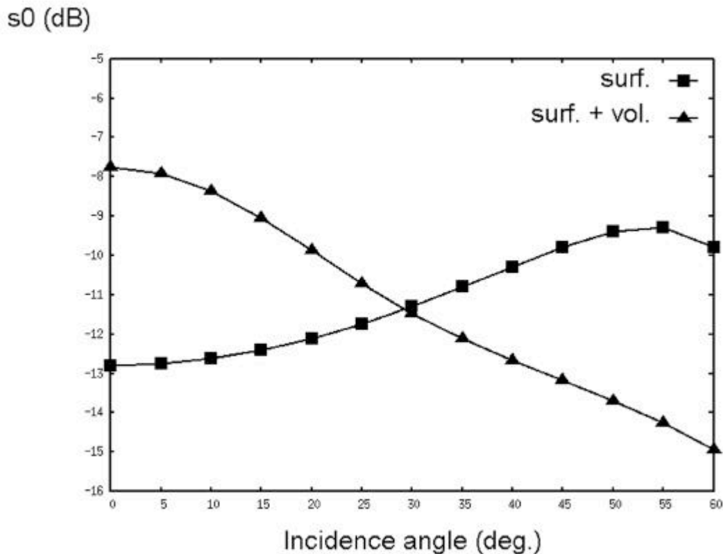
Figure 7: Computed backscattering power for a tholin-composed radar-dark spot with respect to the SAR incidence angle: surface scattering only model (squares) and surface + volume scattering model (triangles).
