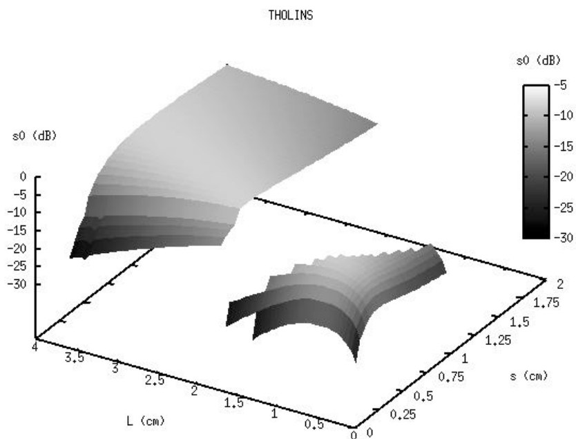
Figure 3: Backscattered power of a single layer of tholins with respect to roughness parameters \sigma and L , at an incidence angle \theta = 30^\circ .
