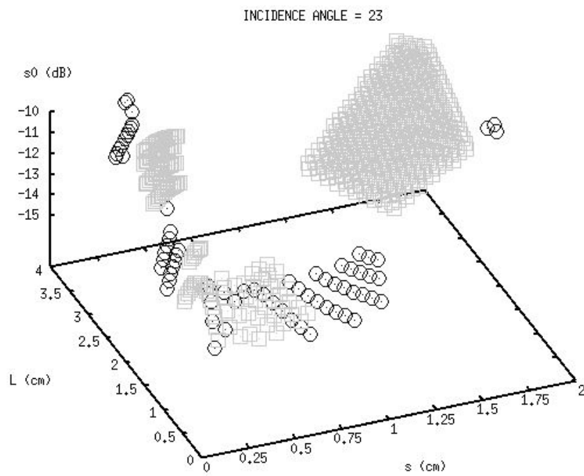
Figure 6: Backscattered power for a single layer of tholins (gray squares) and water-ammonia ice (black circles) with respect to roughness parameters \sigma and L , at incidence angle \theta = 30^\circ (top) and \theta = 23^\circ (bottom).
