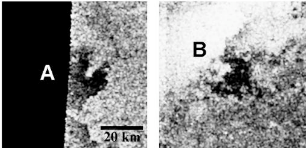
Figure 5: Radar-dark spot A (left) at incidence angle 30^\circ , and B (right) at incidence angle 23^\circ in Ta flyby SAR data.
