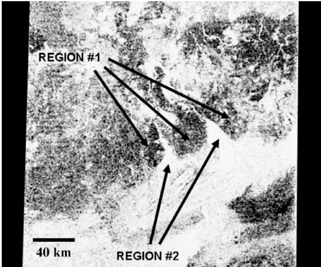
Figure 2: The radar-bright study site located 50.92°N, 79.35°W.
