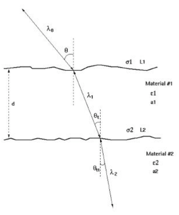
Figure 1: Sketch of the two-layer model of Titan's sub-surface with relevant parameters.
