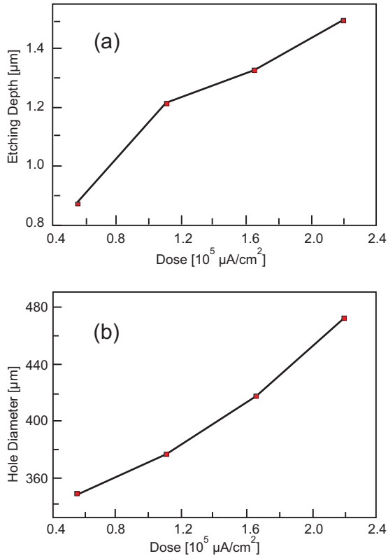
FIG. 4: (a) Dependence of the hole depth with respect to the Ga^+ ion dose with a cross-section at the first hole-line plane. (b) Dependence of the hole diameter with respect to the Ga^+ dose.
