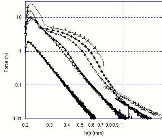
Figure 9: Traction curves for silicone oil G20M at low velocities: V = 0.001\text{mm}\cdot\text{s}^{-1} ( \blacktriangledown ), V = 0.008\text{mm}\cdot\text{s}^{-1} ( \square ), V = 0.01\text{mm}\cdot\text{s}^{-1} ( \blacktriangle ), V = 0.03\text{mm}\cdot\text{s}^{-1} ( \circ ), V = 0.05\text{mm}\cdot\text{s}^{-1} ( \blacklozenge ), V = 0.07\text{mm}\cdot\text{s}^{-1} ( \triangleright ).
