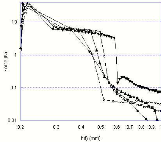
Figure 10: Traction curves for silicone oil G20M at high velocities: V = 0.2\text{mm}\cdot\text{s}^{-1} ( \blacktriangledown ), V = 0.5\text{mm}\cdot\text{s}^{-1} ( \square ), V = 0.7\text{mm}\cdot\text{s}^{-1} ( \blacktriangle ), V = 1.5\text{mm}\cdot\text{s}^{-1} ( \circ ), V = 2\text{mm}\cdot\text{s}^{-1} ( \blacklozenge ).
