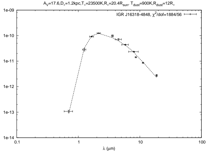
Figure 4. Optical to MIR SED of IGR J16318-4848, including data from ESO/NTT, VISIR on VLT/UT3 and Spitzer (GLIMPSE survey). The observations fitted with both a model of a companion star (taking usual parameters of a sgB[e]) and simple spherical dust component allowed us to derive the following parameters: i) for the companion star: temperature T = 23500 K and radius R_{star} = 20.4R_{\odot} = 15 \times 10^6 km; ii) for the dust component: temperature T = 900 K, radius R = 12R_{star} = 171 \times 10^6 km. The absorption we derived was A_v = 17.6 magnitudes, and the distance D = 1.2 kpc. The high \chi^2/\text{dof} value of the fit ( =1884/56 ) is mainly due to the very small error bars in the MIR domain. The main result given by this SED is that in the case of IGR J16318-4848 there is a need for an extra (e.g. dust) component in order to fit its SED.
