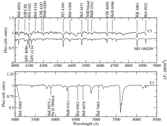
Figure 5. Optical spectrum of IGR J17544-2619 showing the identified lines, among which Pellizza et al. (2006) found strong HI, HeI and HeII lines typical of an O-type star. Upper panel: Blue spectrum of IGR J17544-2619 (upper curve) and the standard O9Ib star HD 188209. The high degree of similarity between them supports their classification of IGR J17544-2619 as an O9Ib star. Lower panel: Spectrum of IGR J17544-2619 between 5000 Å and 8500 Å.
