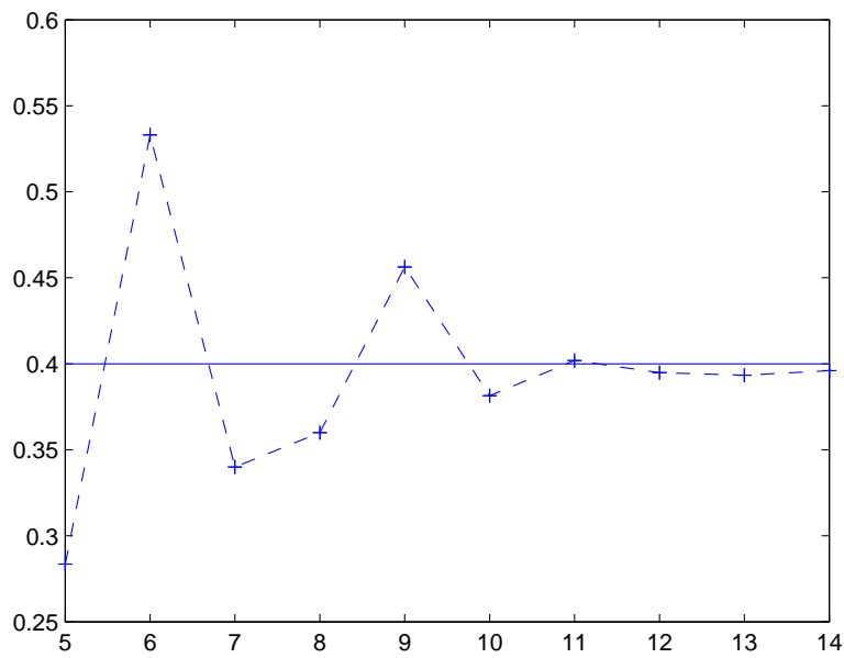
Figure 3: Estimator of H = .4
