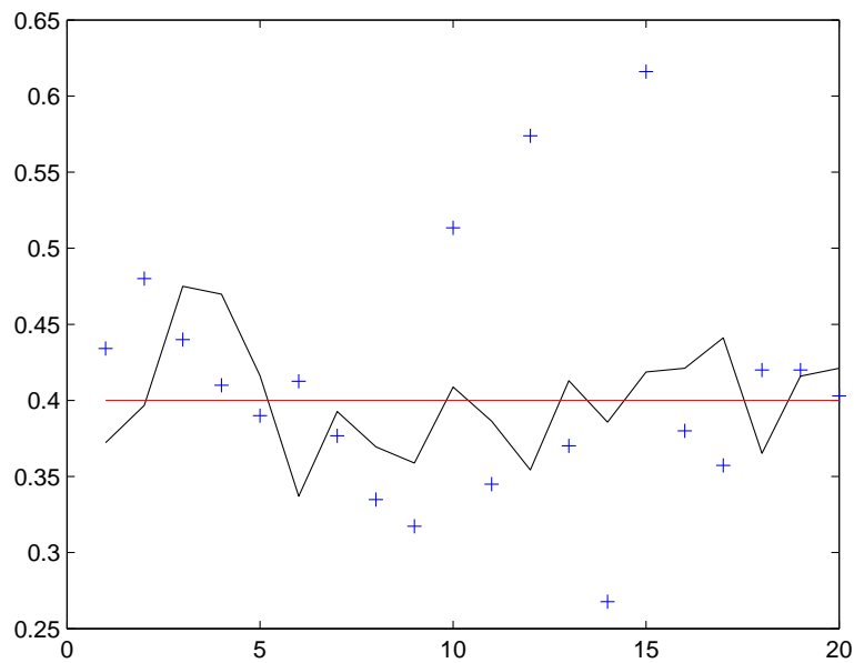
Figure 5: Comparison of Estimators with true observations
