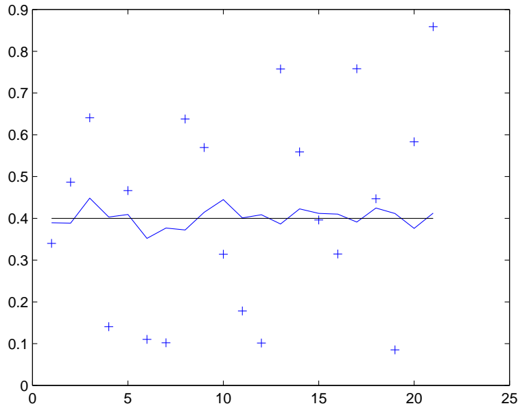
Figure 6: Comparison of Estimators with noisy observations
