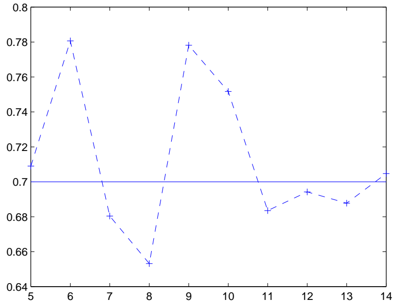
Figure 4: Estimator of H = .7
