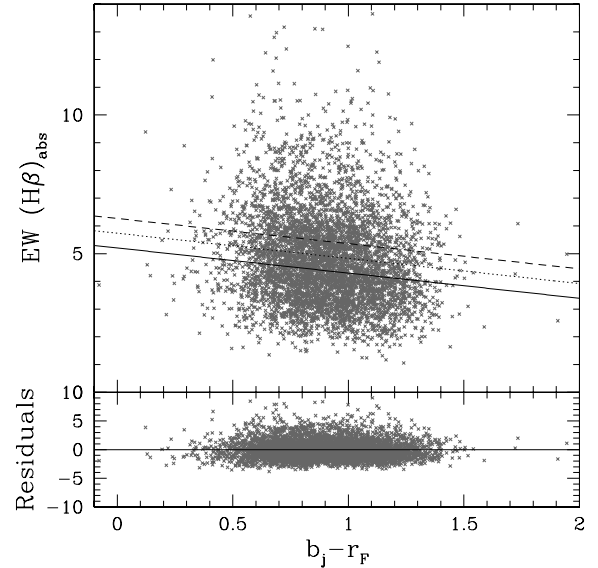
Figure 5. Variation of EW(\text{H}\beta)_{\text{abs}} as a function of (b_j - r_F) colour (top panel) for our sample of starburst galaxies, restricted to galaxies with a good fit of \text{H}\beta absorption line. Solid, dotted and dashed lines show the empirical calibration found for M_B = -24 , -18 and -12 , respectively. The bottom panel shows the residuals versus the (b_j - r_F) colour; their rms is 1.75 \text{ \AA} .
