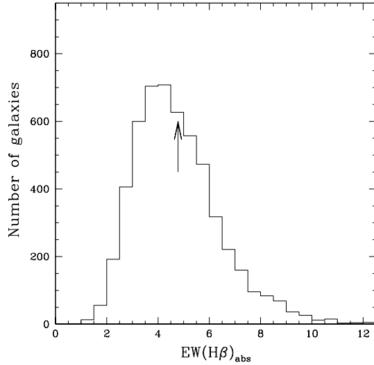
Figure 4. Distribution of the EW of \text{H}\beta in absorption restricted to galaxies with a good fit quality. The arrow indicates the mean value EW(\text{H}\beta)_{\text{abs}} = 4.6 \text{ \AA} of the sample.
