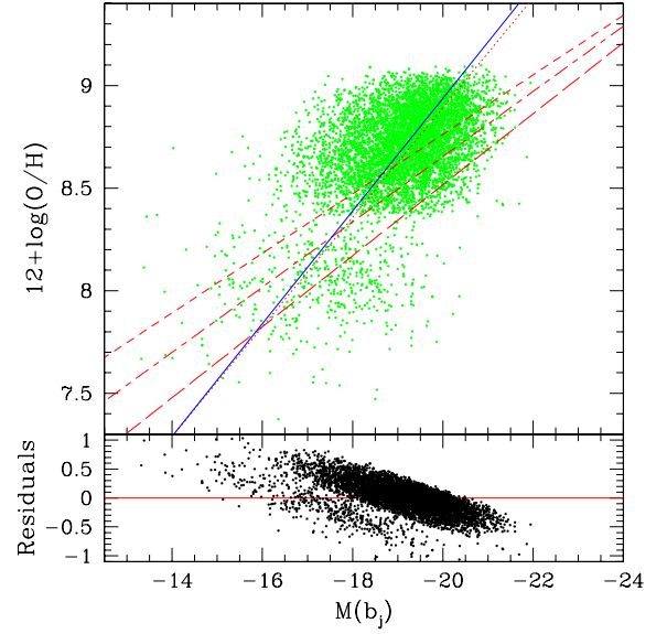
Figure 6. L–Z relation for the sample of 6387 star-forming galaxies extracted from the 2dFGRS. The linear regression on this sample is plotted as a solid line. The dotted line shows the relation from Melbourne & Salzer (2002), the short-dashed line the relation for normal galaxies (Kobulnicky et al. 1999), the long-dashed line for UV-selected and H II galaxies (Contini et al. 2002) and the short-dashed–long-dashed line the relation for spirals from Pilyugin et al. (2004). The bottom panel shows the residuals of the linear regression.
