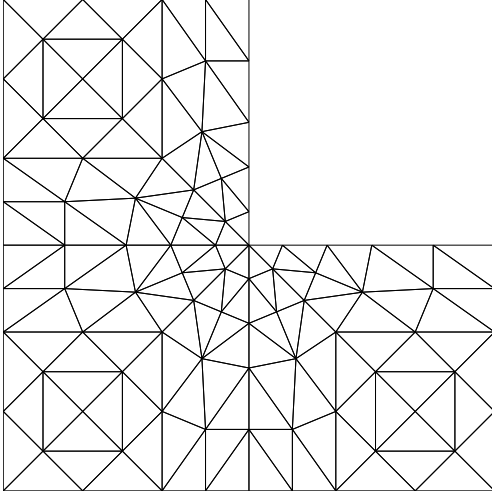
Figure 8.1: Graded mesh for h = 0.125 and \mu \approx 0.533
