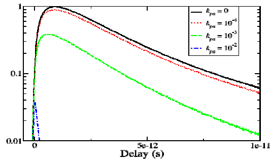
Fig. 7. Relative scattered intensity as a function of TOF for different values of k_{pa} and for a 5 \mu m particle radius.
