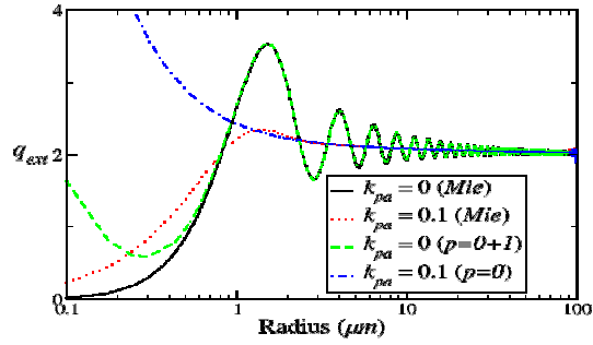
Fig. 5. Extinction efficiency q_{\text{ext}} (Eq. (6)) as a function of the particle radius. Total (solid black and dotted red lines) and partial (dotted green and blue lines) extinction efficiencies are plotted for different values of k_{pa} .
