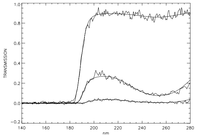
Figure 8. Three examples of transmission profiles and corresponding fit results obtained with a Levenberg-Marquardt fit algorithm. The CO 2 absorption is dominant below 190 nm. The corresponding altitudes are around 10 km, 30 km, and 50 km. Ozone absorption is seen for all these altitudes in that particular case.
