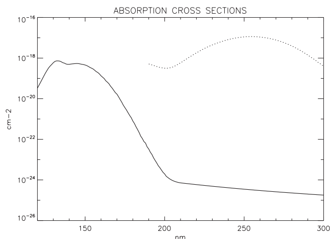
Figure 5. Absorption cross sections of CO 2 (thick line) and O 3 (dotted line) used in the inversion [from Yoshino et al. , 1996]. In the inversion we have assumed that the cross sections do not depend on temperature. The values shown here correspond to a temperature of 195 K. Cross-section values are averaged on a 1-nm interval to account for the spectrometer resolution. A sliding mean over 3 pixels has also been performed to account for the point spread function of the spectrometer. In the case of CO 2 , Rayleigh scattering extinction is added and becomes important above 210 nm.
