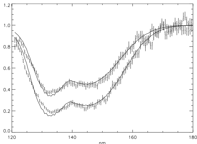
Figure 6. Typical transmission spectra above 100 km used to perform the wavelength assignment. Transmissions for 2 altitudes are plotted. The data (dotted line) are shown with statistical errors. The solid lines show the modeled transmission. Because the star is not always at the center of the field of view, we need to determine the possible shift of the observed spectra on the CCD. This is done by fitting the data with models using the CO 2 cross section shown in Figure 5, because only CO 2 has a significant absorption above 100 km altitude. We allow for an unknown shift on the x axis and determine its value in the fit. This is a sensitive indicator because of the small bumps in transmission around 140 nm.
