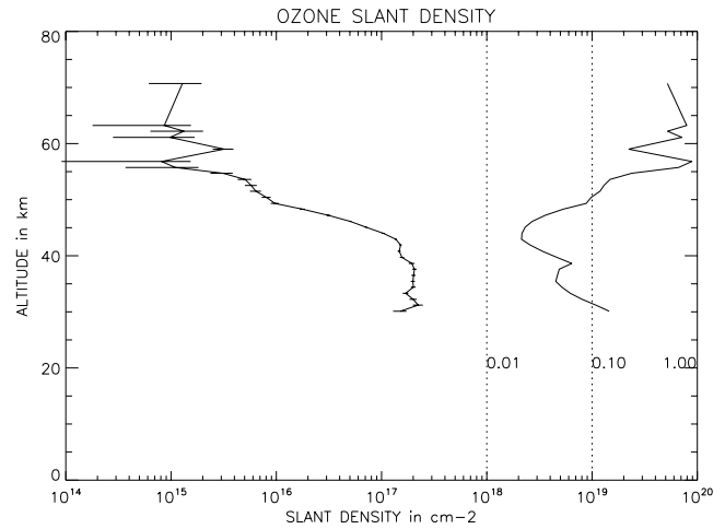
Figure 10. Vertical profile of ozone slant density in \text{cm}^{-2} obtained from the same occultation as in the previous figure. Here ozone absorption becomes marginal above 45 km. At lower altitudes the accuracy is limited by the amount of aerosols in the atmosphere. Relative uncertainties are shown on the right-hand panel. They range between 0.01 and 1.00.
