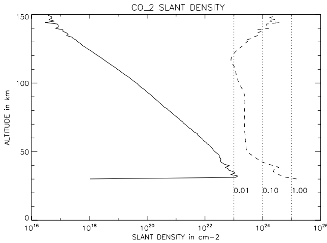
Figure 9. Vertical profile of \text{CO}_2 slant density in \text{cm}^{-2} obtained from one occultation. This is obtained by assuming that the absorption cross section of \text{CO}_2 is independent of temperature. Relative error bars resulting from the Levenberg-Marquardt algorithm are displayed on the right-hand panel. They are very small in the range 45–130 km, covering a dynamic range of 10^5 in slant density of \text{CO}_2 . This is possible because of the huge variation of \text{CO}_2 cross section in the wavelength range 130–200 nm covered by SPICAM.
