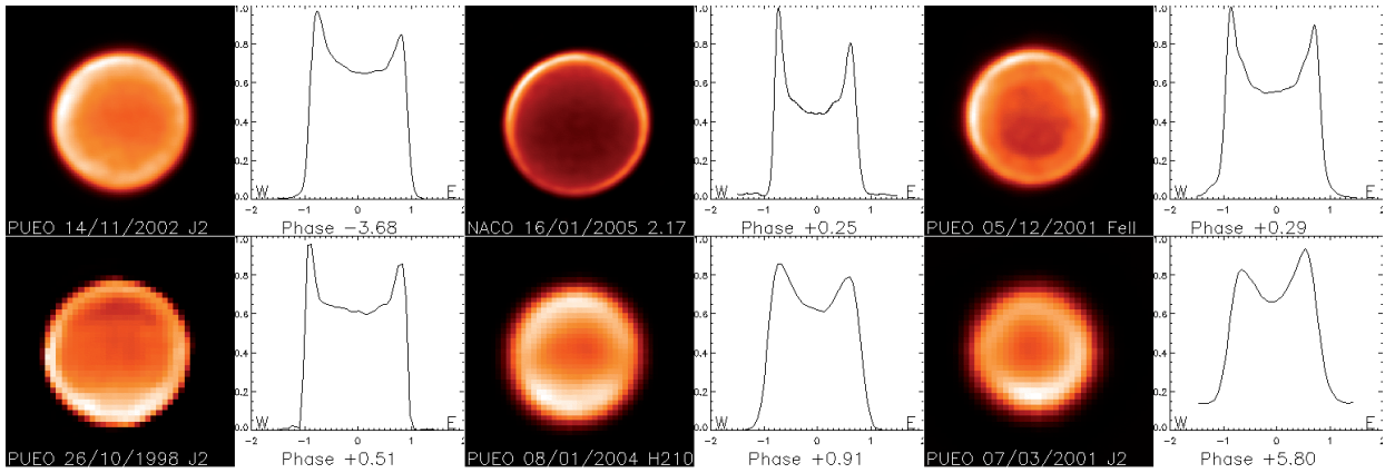
Fig. 3. Typical AO images showing the evolution of the east-west asymmetry on Titan as a function of solar phase angle, regardless of the actual date of observation (reported on the bottom of each image, along with the instrument used and the solar phase angle value). From upper left to bottom right, the solar phase angle increases, showing the reversal of the phase effect from the morning (west, left ) to the evening (east, right ) sides. The profiles drawn correspond to normalized intensity (1 being the brightest pixel of the image) from one limb to another, along one parallel, the one where the effect is maximum returning the nominal value reported in Table 3. At large phase angle values, the brightest limb corresponds to the sunlit one: western at negative phase angles ( upper left ), eastern at positive angles ( bottom right ). Yet at low phase angle values (the four intermediate cases: upper centre , upper right , bottom left and bottom centre ), the western limb (morning side) is always brighter than the eastern one (evening side), characteristic of a morning haze enhancement phenomenon related to a nocturnal condensation of stratospheric aerosols. See text for more details.
