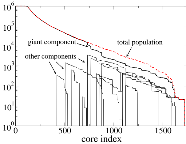
FIG. 9: Color online: Plot of the number of particles in disconnected components in each core, as a function of the core index, at time \tau = 200 cpp. At small core indexes, the number of observed disconnected components is 1, then it grows up to \sim 6 .
