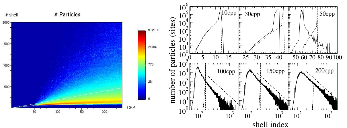
FIG. 8: Color online: Distribution of k -shells in the large inelastic system against time \tau measured in collisions per particle (cpp). Left: time is on the x -axis, while shell index k is on the y -axis. Brightness/color indicates population (number of particles in the shell). The solid white line marks the 1.8\tau law observed in the homogeneous case. Right: sections of the left graph at six different times (solid line), compared with the elastic system of same size (light dashed lines). The bold dashed line marks a power law decay with -3 exponent.
