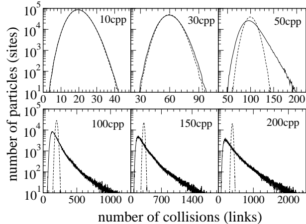
FIG. 7: Histograms of degree distribution f(d, \tau) for different values of \tau , i.e. of number of collisions per particle: comparison between the large inelastic system (solid line) and the elastic system (dashed line).
