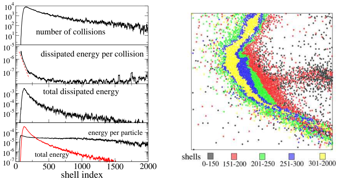
FIG. 10: Color online. Left: statistics of physical observables in different shells at a given time ( \tau = 200 cpp). Topmost graph: number of collisions performed by particles in a given shell. Second graph from top: dissipated energy per collision, together with an exponential fit of the first decay \sim \exp(-0.03k) . Third graph: dissipated energy summed over all collisions done by particles in a given shell. Fourth graph: average energy competing to each particle in a given shell and total energy contained in a given shell, rescaled in order to appear on the same scale. Right: a snapshot of the system at \tau = 200 cpp, showing in different colors the shell each grain belongs to.
