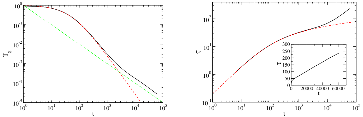
FIG. 2: Color online: Left: decay of granular temperature T_g vs. time t . The dashed red line marks the Haff law, T_g = 1/(1 + t/t_e)^2 with t_e \approx 52 , the dotted green line is a t^{-1} decay. Right: cumulated number of collisions per particle \tau vs. time t , the dashed red line shows the logarithmic growth of collisions in the Haff phase, \tau = a \log(1 + t/t_e) with a \approx 10 . In the inset a linear plot of \tau vs. t is shown, focusing on the behavior at large times ( t \gg 10^4 ). The system is a gas of N = 10^6 inelastic hard disks with restitution coefficient \alpha = 0.9 in a box of size 3163 \times 3163 (units of a diameter) with periodic boundary conditions. Averages over 10 different initial conditions have been performed.
