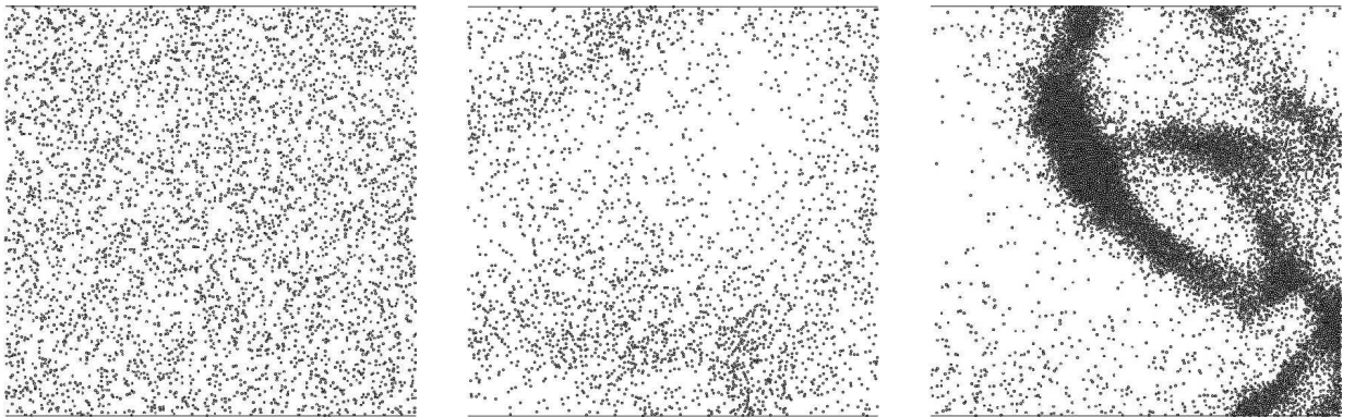
FIG. 3: Three snapshots of a small part of the gas of 10^6 inelastic hard disks with restitution coefficient \alpha = 0.9 . In the snapshots is portrayed a square of surface 200 \times 200 , in units of a diameter, where the whole system is 3163 \times 3163 ; therefore the pictures portray a fraction 0.004 of the total surface. Left: just after thermalization (0 cpp). Center: after 100 cpp (collisions per particle). Right: after 200 cpp.
